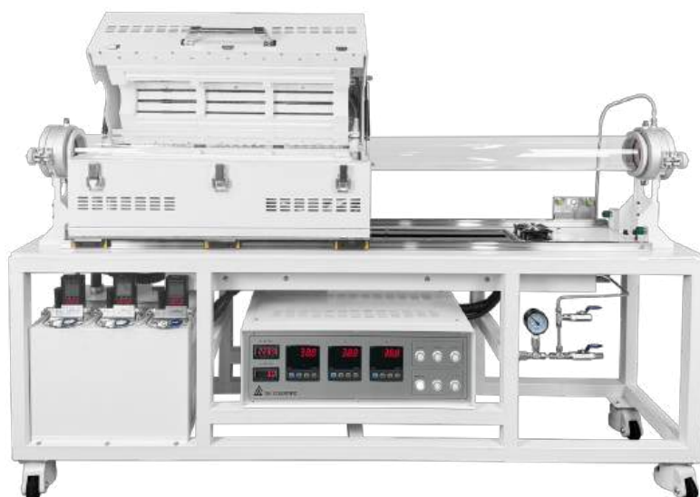
RTCVD Tube Furnace (Gas Flow Package)
