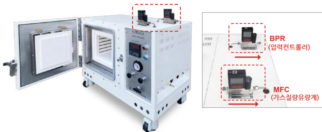
Muffle Furnace with Vacuum
